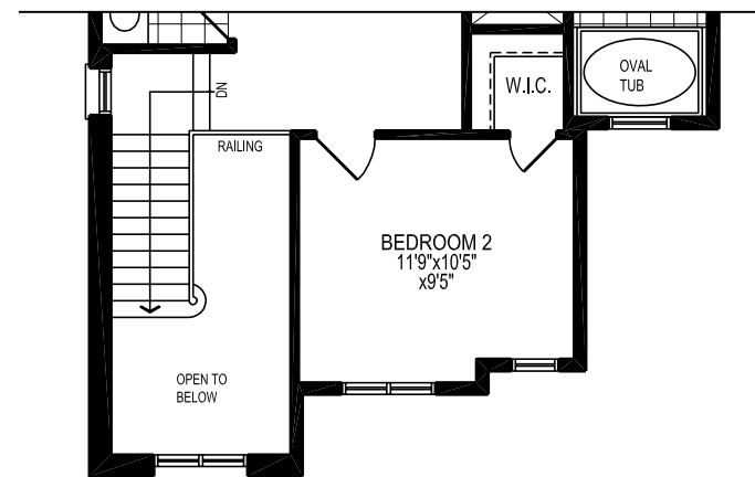
PARTIAL SECOND FLOOR PLAN 'B'
