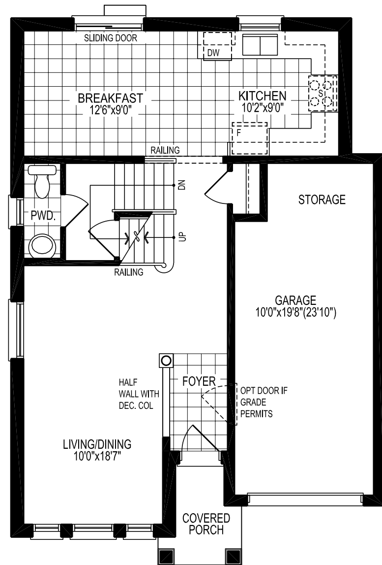
GROUND FLOOR PLAN 'A'
