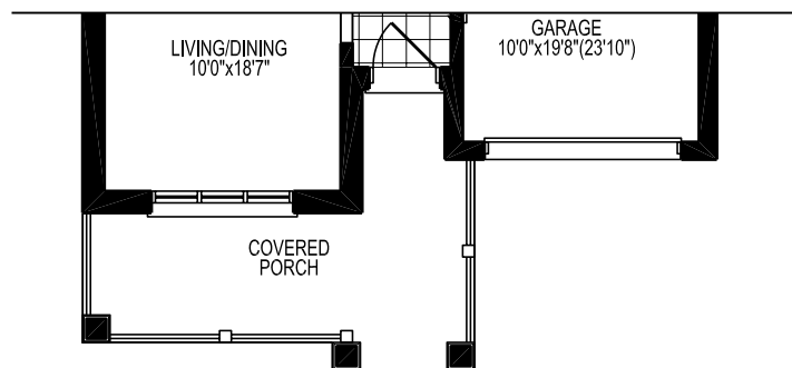
PARTIAL GROUND FLOOR PLAN 'B'
