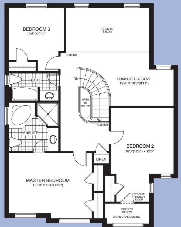
Upper Level Alternate layout
