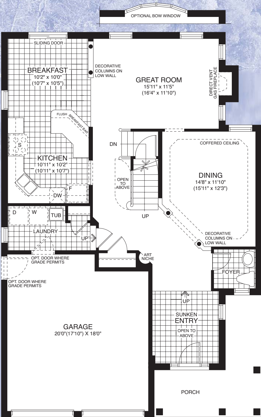
Main Level Elevation A&B
